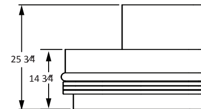
STEPS SECTION
